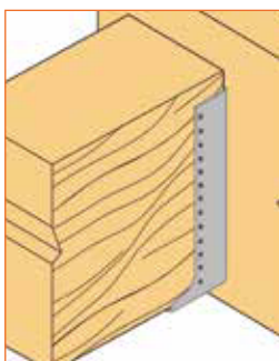
GLI : Fixation sur support BOIS Clouage total
